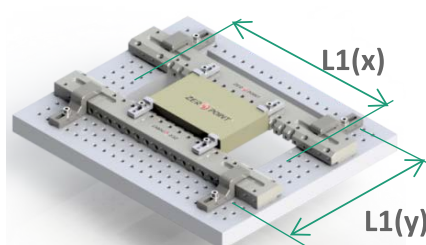
① Large work Piece
