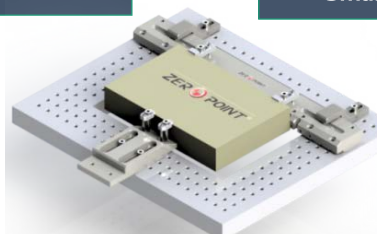
①+④ Medium-Large work Piece
