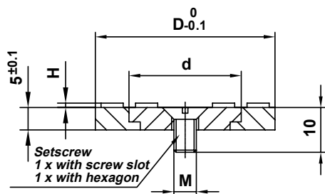
Dati 4400 from Ms 58 | Dati 4000 from 1.2510 HRC 54 engraving raised
