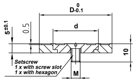
Dati 4600 from Ms 58 | Dati 4500 from 1.2510 HRC 54 engraving recessed
