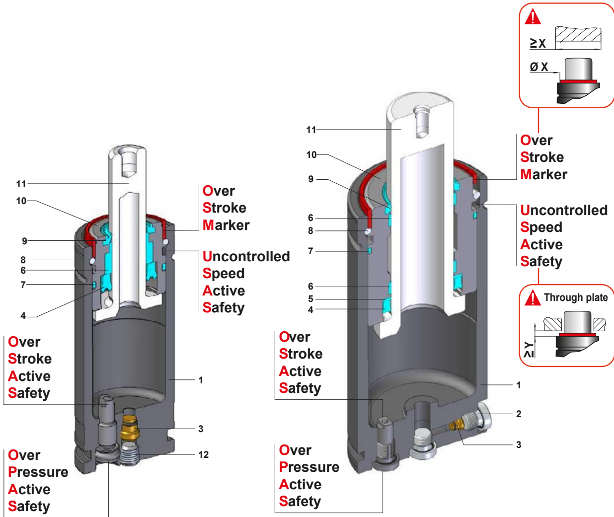
SC 150 ÷ SC 10000
