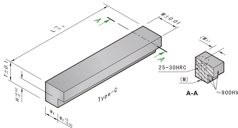
KDT1475-T-H-L M Material:P20 H Hardness:≈900HV
