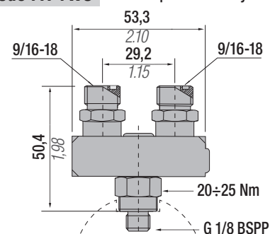
code PA-TWS Port Adapter - Two Way Swivel
