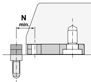
Slide Disassembling
