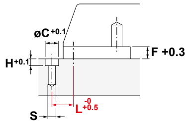
Mold Open
