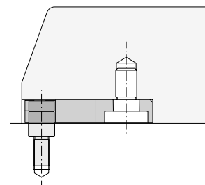
Mold Open
