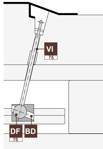
Angled Undercuts
